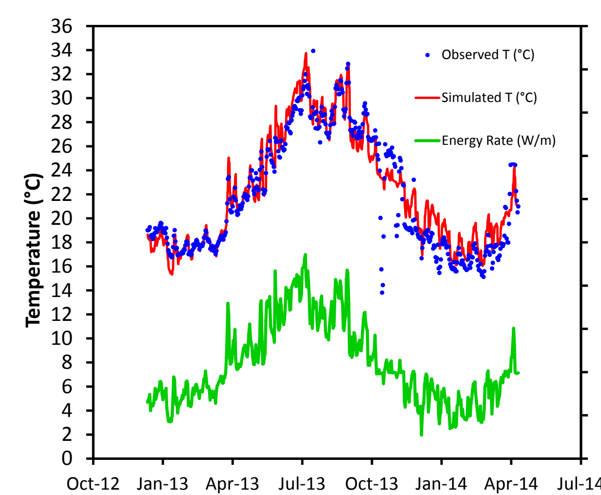
Figure 5. Computer-simulated (red) and observed (blue) daily ground temperature calculated from system heat flux (green) Dec 2012 to present.
