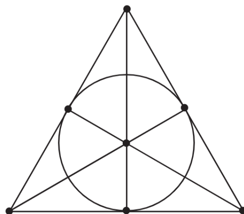
The Fano Plane
