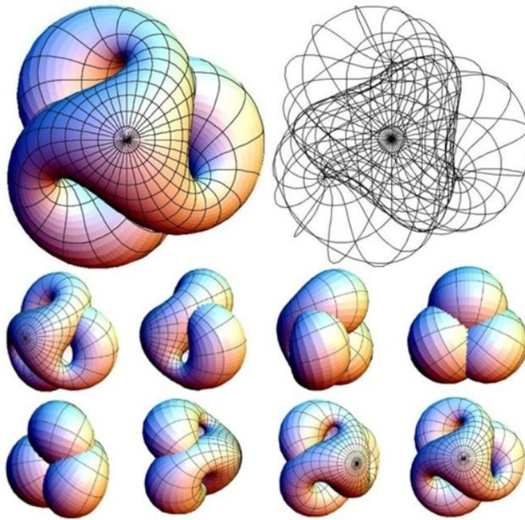
Boy's Surface (representation of the projective plane)
